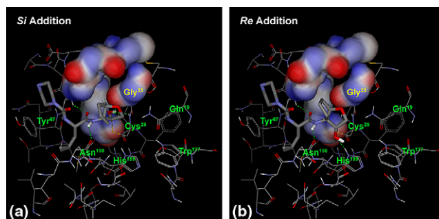
Figure 5. Predicted binding conformations for si (a) and re (b) stereofacial thiolate addition to a model bicycle 5 , (3 aR ,6 aR ) piperazine-1-carboxylic acid [3-methyl-1 S -(3-oxo-hexahydrocyclopenta[ b ]furan-3-yl-carbamoyl)butyl]amide. 9,10a The residues Gly 23 , Trp 26 , Cys 63 , Gly 64 and Gly 65 that make the P1 wall of cathepsin K structure 1mem are shown as an electrostatic potential coloured surface. The hydrogen atoms of the intermediate hydroxyl, ring bridgehead 6a and -NH are added.
