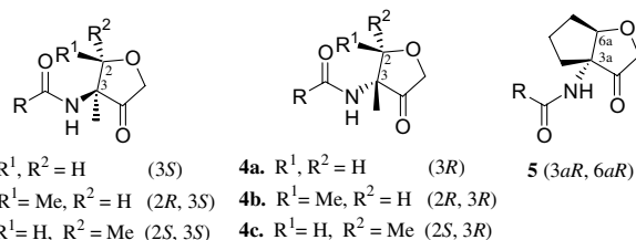
Figure 2. Stereochemical assignment of \alpha,\beta -dimethyl monocyclic and N -(3-oxo-hexahydrocyclopenta[ b ]furan-3a-yl)acylamide bicyclic ketone inhibitors of CAC1 cysteinyl proteinases.
