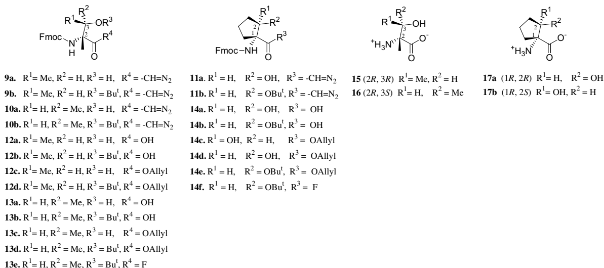
Figure 7. Amino acid building blocks towards mono- and bicyclic scaffolds 6–8 .
