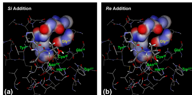
Figure 3. Predicted binding conformations for si (a) and re (b) stereofacial thiolate addition to a model \alpha -methyl monocyclic 3a , piperazine-1-carboxylic acid [3-methyl-1 S -(3 S -methyl-4-oxo-tetrahydrofuran-3-yl-carbamoyl)butyl]amide. 9,11 The residues Gly 23 , Trp 26 , Cys 63 , Gly 64 and Gly 65 that make the P1 wall of cathepsin K structure 1mem are shown as an electrostatic potential coloured surface. The hydrogen atoms of the intermediate hydroxyl, \alpha -methyl and \alpha -NH are added and residue Gly 23 labelled.
