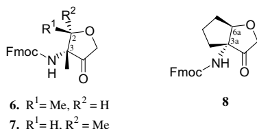
Figure 6. Protected mono- and bicyclic building blocks towards solid-phase assembly of compounds of general formulae 4 and 5 .
