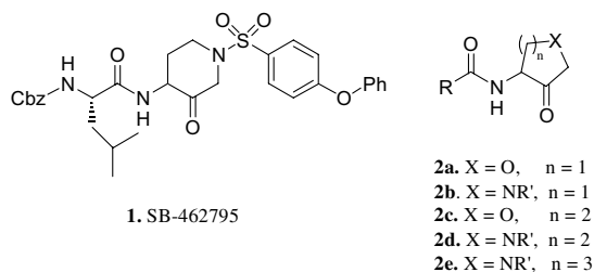
Figure 1. GSK cyclic ketone inhibitors of cathepsin K.
