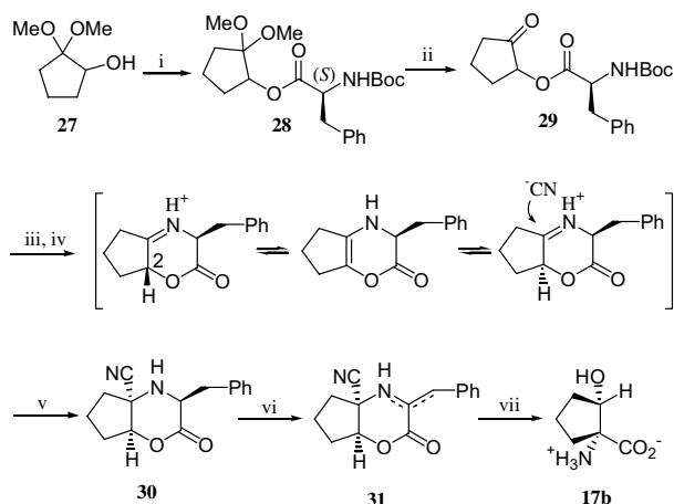
Scheme 3. Synthesis of 17b . Reagents and conditions: (i) BocPheOH, EDC, DMAP, dichloromethane; (ii) para -toluenesulfonic acid monohydrate, (CH 3 ) 2 CO; (iii) TFA, CH 2 Cl 2 , then concentration in vacuo and azeotropic removal of excess TFA with toluene; (iv) MgSO 4 , NaOAc, CH 3 CN, then filtration and concentration in vacuo; (v) TMSCN, ZnCl 2 ; (vi) 2 equiv tert -BuOCl, Et 2 O, followed by triethylamine; (vii) cHCl, Dowex® 50W×4 (elution with 1 M NH 3 ).
