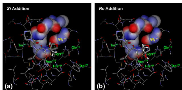
Figure 4. Predicted binding conformations for si (a) and re (b) stereofacial thiolate addition to a model \alpha -methyl monocyclic 4a , piperazine-1-carboxylic acid [3-methyl-1 S -(3 R -methyl-4-oxo-tetrahydrofuran-3-yl-carbamoyl)butyl]amide. 9,11 The residues Gly 23 , Trp 26 , Cys 63 , Gly 64 and Gly 65 that make the P1 wall of cathepsin K structure 1mem are shown as an electrostatic potential coloured surface. The hydrogen atoms of the intermediate hydroxyl, \alpha -methyl and \alpha -NH are added and residue Gly 23 labelled.
