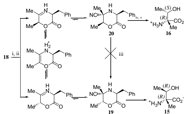
Scheme 1. Synthesis of (2 R ,3 S )- 16 . Reagents and conditions: (i) TFA, \text{CH}_2\text{Cl}_2 ; (ii) 2 equiv powdered NaCN, 2-propanol, 2 h; (iii) 1 equiv TFA, 2-propanol then recrystallisation from \text{Et}_2\text{O} /hexane; (iv) 2 equiv tert -BuOCl, \text{Et}_2\text{O} , then triethylamine; (v) cHCl; Dowex ® 50W×4 (elution with 1 M \text{NH}_3 ), then recrystallisation from \text{H}_2\text{O} /EtOH/ \text{Et}_2\text{O} .
