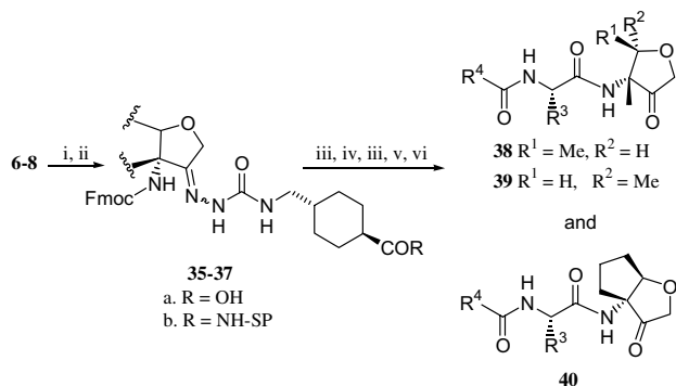
Scheme 4. Synthesis and use of supported linker constructs 35b–37b . Reagents and conditions: (i) trans -4[(hydrazinocarbonyl)amino]methylcyclohexanecarboxylic acid, trifluoro-acetate, EtOH, H 2 O, NaOAc, reflux; (ii) 3 equiv 35a–37a , 3 equiv HBTU, 3 equiv HOBt, 6 equiv NMM, H 2 N-solid phase, DMF; (iii) 20% piperidine/DMF (v/v), 30 min; (iv) 10 equiv Fmoc-NHCHR 3 -COOH, 10 equiv HBTU, 10 equiv HOBt, 20 equiv NMM, DMF, rt, o/n; (v) 10 equiv R 4 -COOH, 10 equiv HBTU, 10 equiv HOBt, 20 equiv NMM, DMF, rt, o/n; (vi) TFA/H 2 O, (95:5, v/v), rt, 2 × 24 h ( 35b , 36b ), 1 × 24 h ( 37b ).
